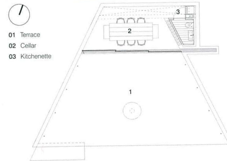
FLOOR PLAN
